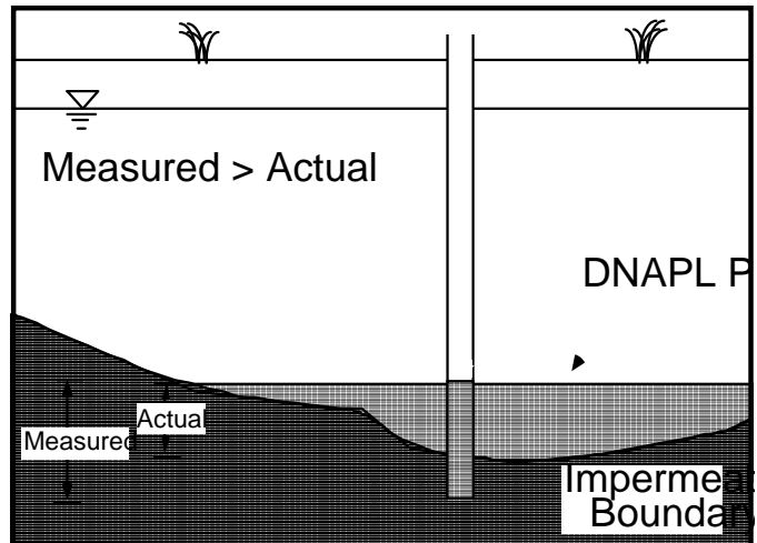
Figure 19. A well screened into an impermeable boundary may result in an over-estimation of the DNAPL thickness.
