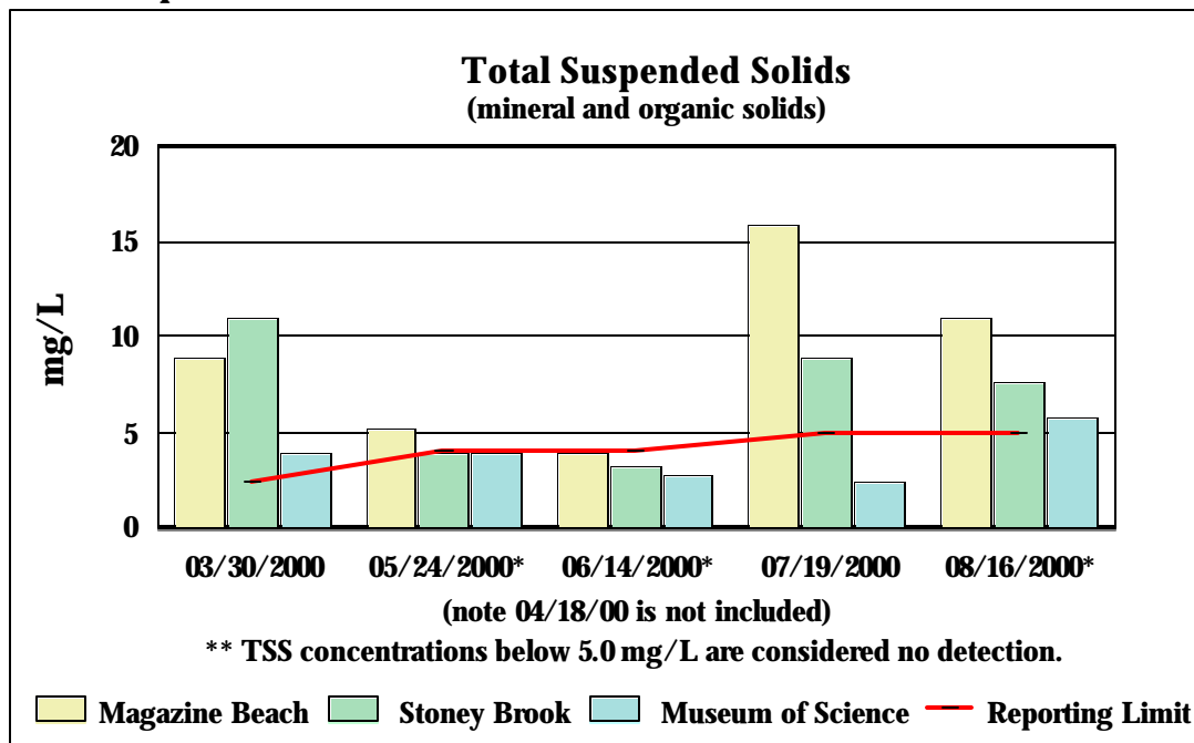
Figure 3. Total Suspended Solids Measurements for the Three Lower Basin Sites
