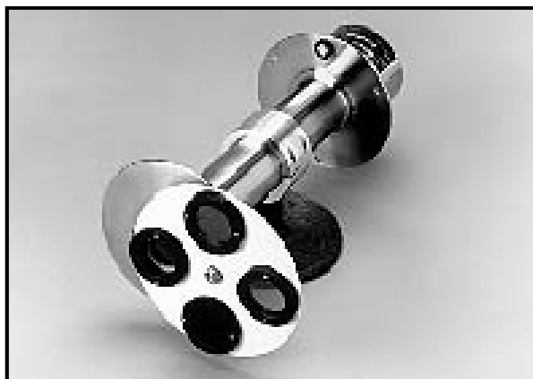
Figure 6.6 Eppley Normal Incidence Pyrheliometer
