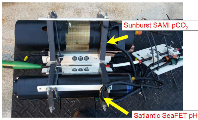
Long Island Sound instrument array
