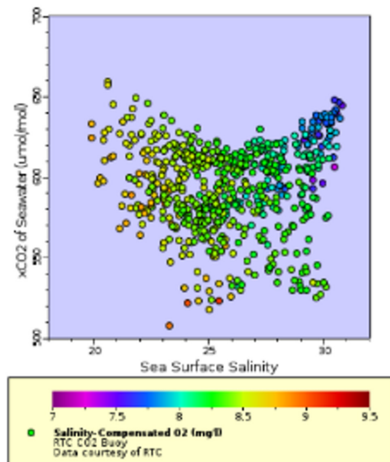
Figure 24. San Francisco Estuary–Ocean and watershed sources of high p\text{CO}_2
