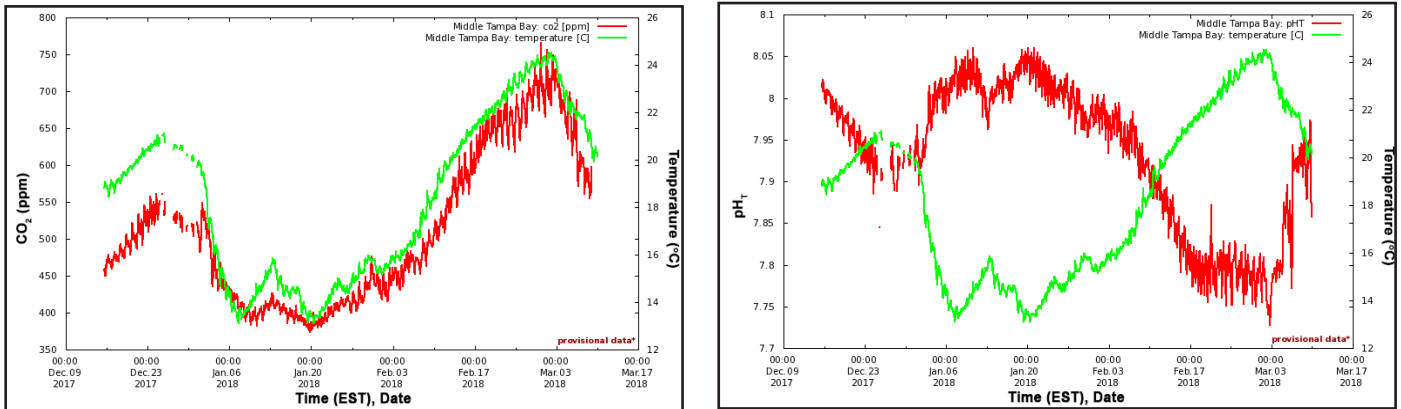
Figure 16. Tampa Bay – pH and p\text{CO}_2 and Temperature (December 2017 to March 2018).
