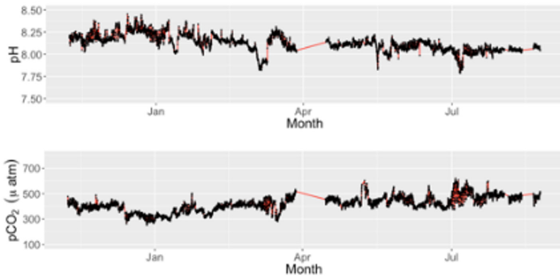
Figure 17. Coastal Bend Bays – pH and p\text{CO}_2 data during the deployment period. The black data points represent hourly measurements. Gaps between points occur when there were outliers due to various reasons.
