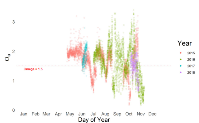
Figure 10. Aragonite Saturation State 2015–2018. Casco Bay.
