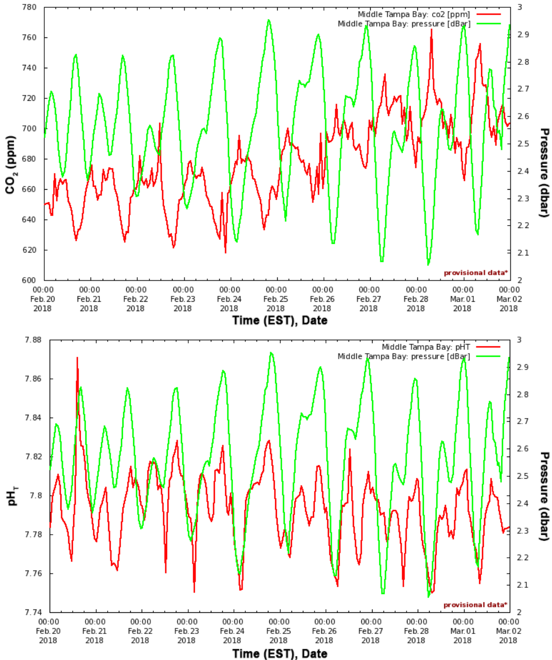
Figure 15. Tampa Bay—pH and p\text{CO}_2 at Middle Tampa Bay in February and March 2018.
