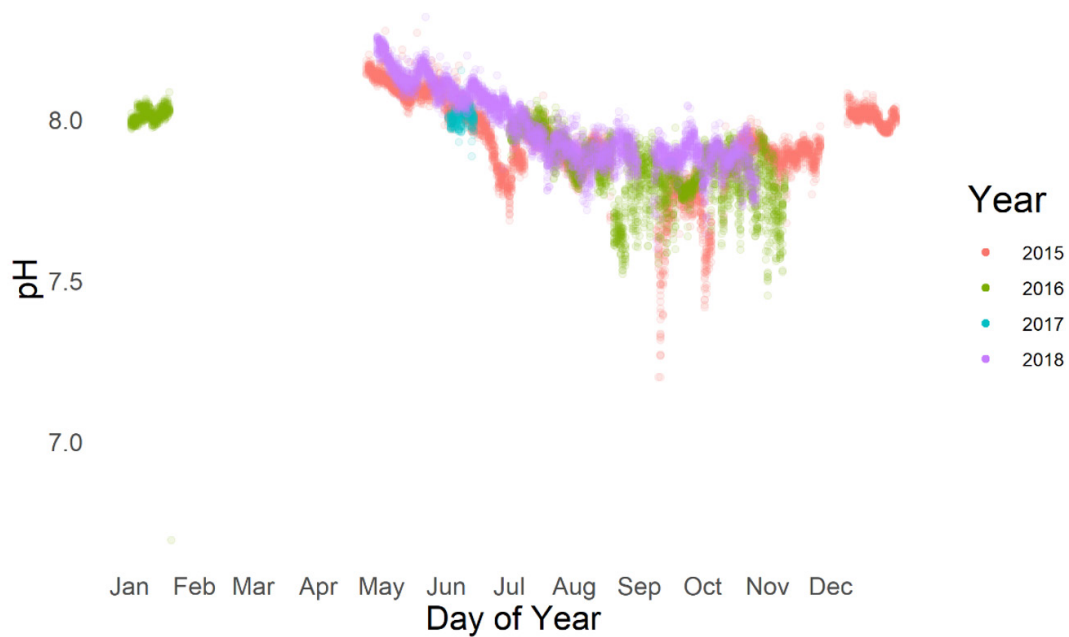
Figure 5. Observed pH increases in the spring and decreases in the fall. Casco Bay.
