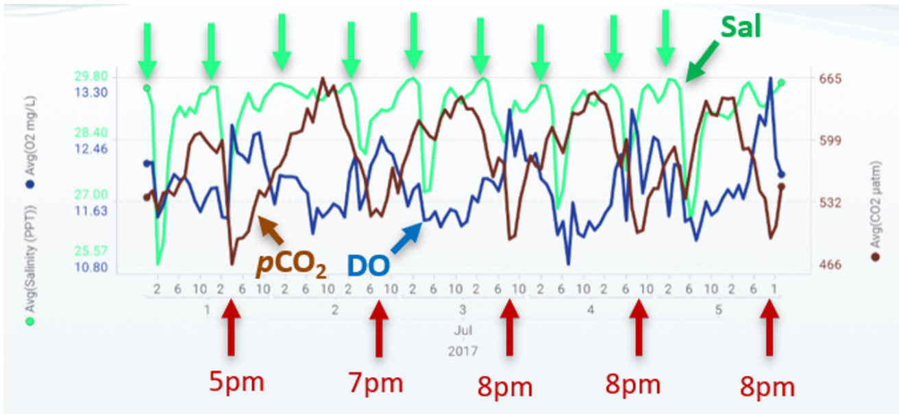
Figure 7. Observed daily variability of p\text{CO}_2 , DO, and salinity (July 1-5, 2017).
