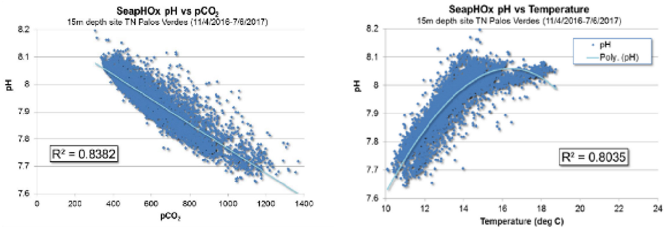
Figure 21. Santa Monica Bay—Relationship of pH and p\text{CO}_2 (left) and pH and temperature (right) in Year 1
