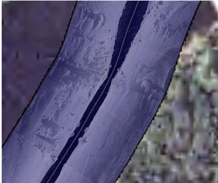
Figure 3-3. Example of sonar imagery acquired along mid-pool habitat using a beam set to record on each side during the habitat survey of the Merrimack River, 16 September through 2 November 2010.
