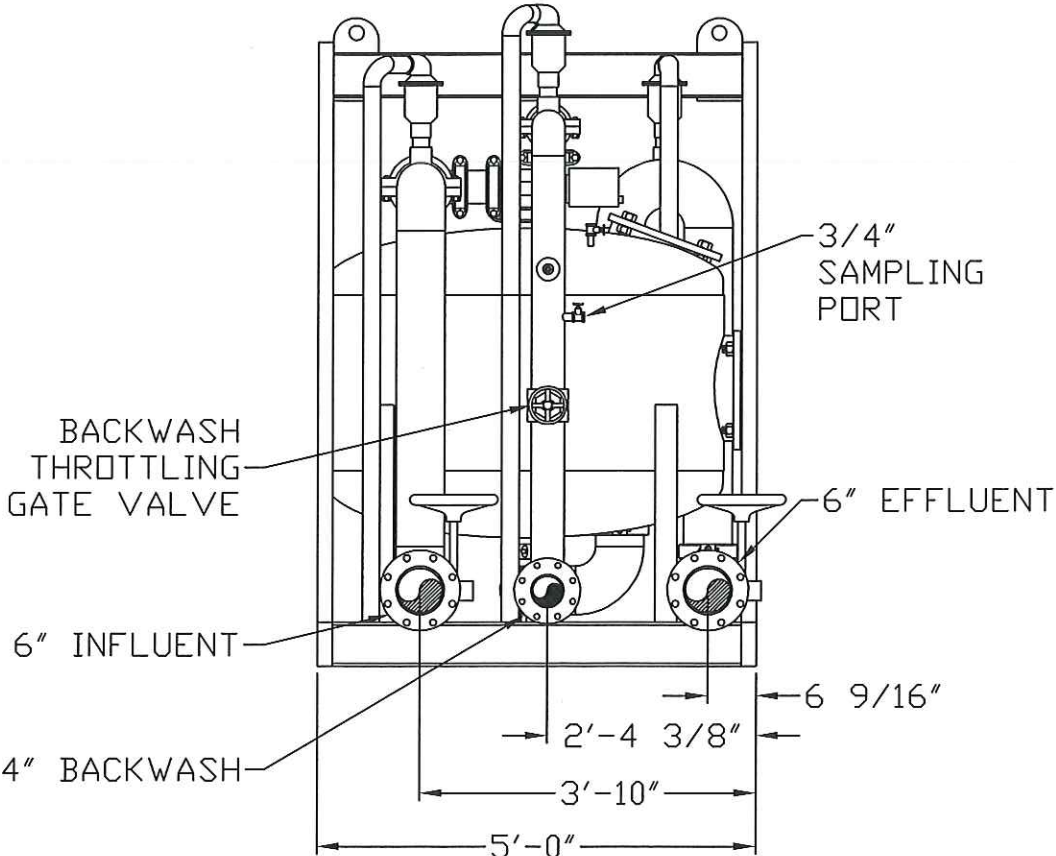
END VIEW
