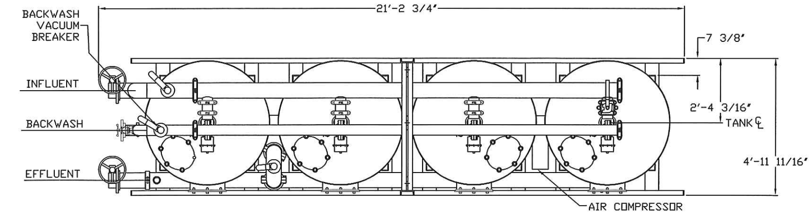
TOP VIEW
