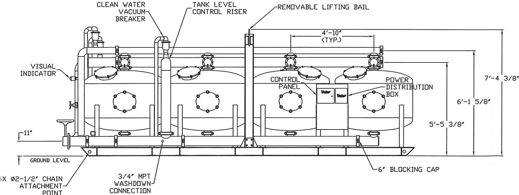
SIDE VIEW
