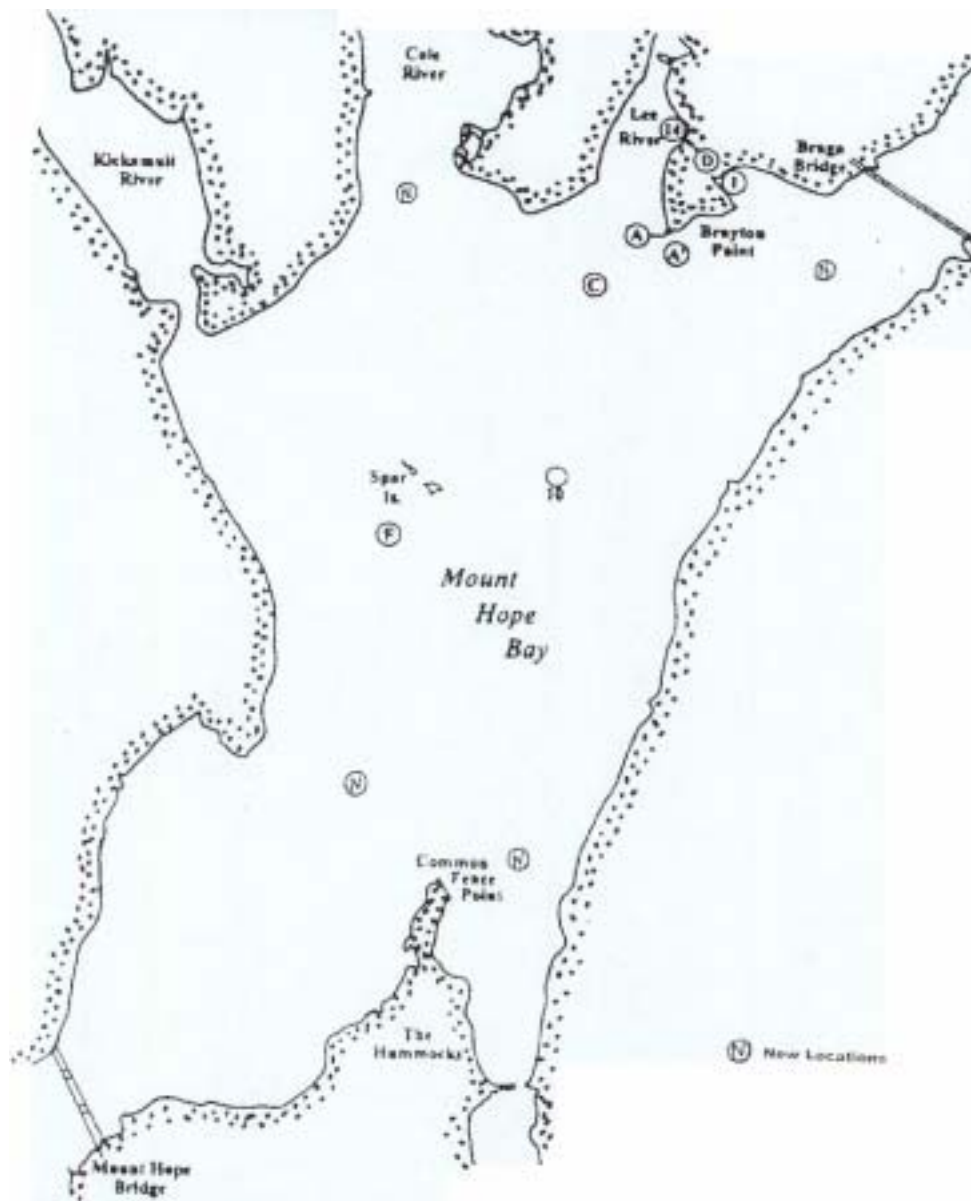
Figure 6: Location of Thermistors for Water Temperature Monitoring in Mount Hope Bay
