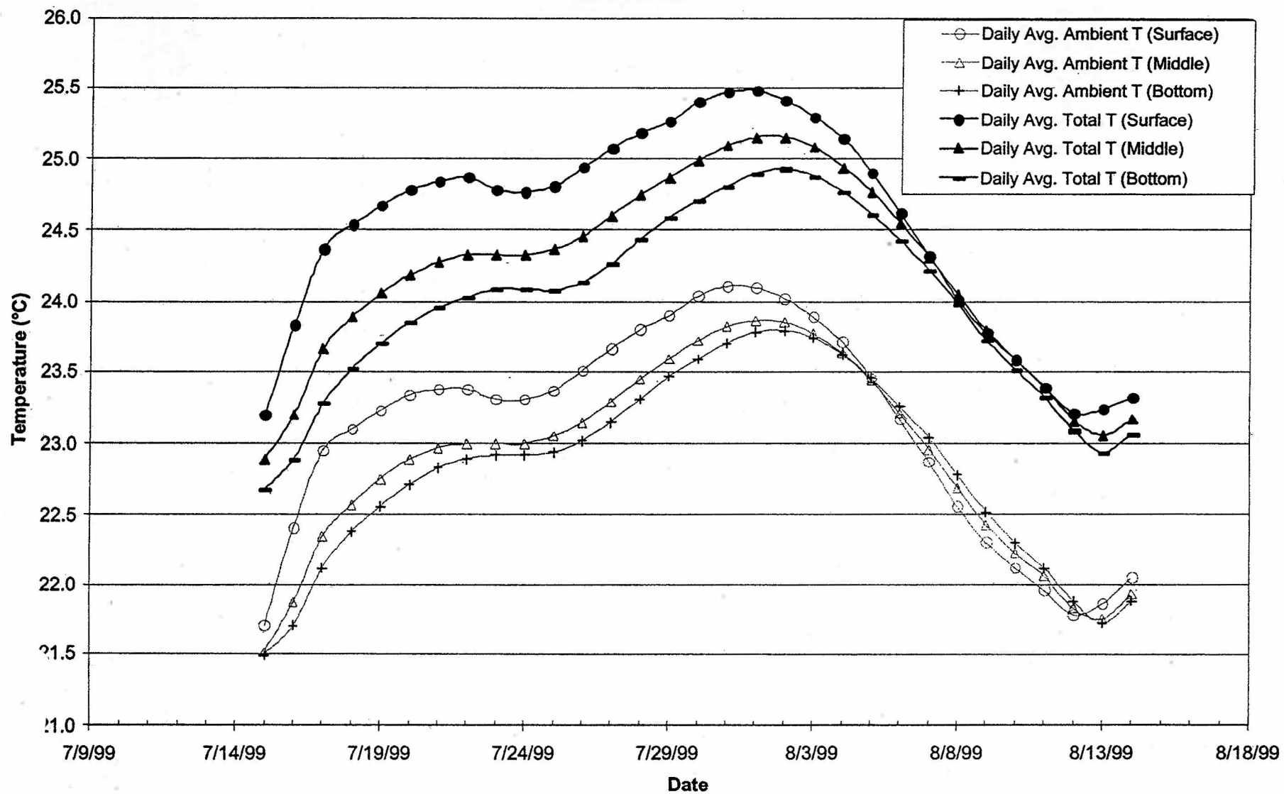
Figure 17: "Translation" of Delta T Results to Average Ambient and Total Temperature (Summer 1999, Enhanced Multi-Mode Scenario)
