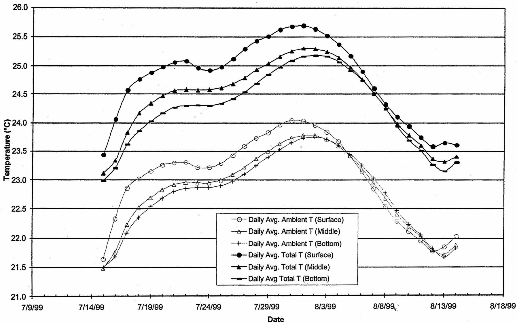
Figure 16: "Translation" of Delta T Results to Average Ambient and Total Temperature (Summer 1999, MOA II Scenario)
