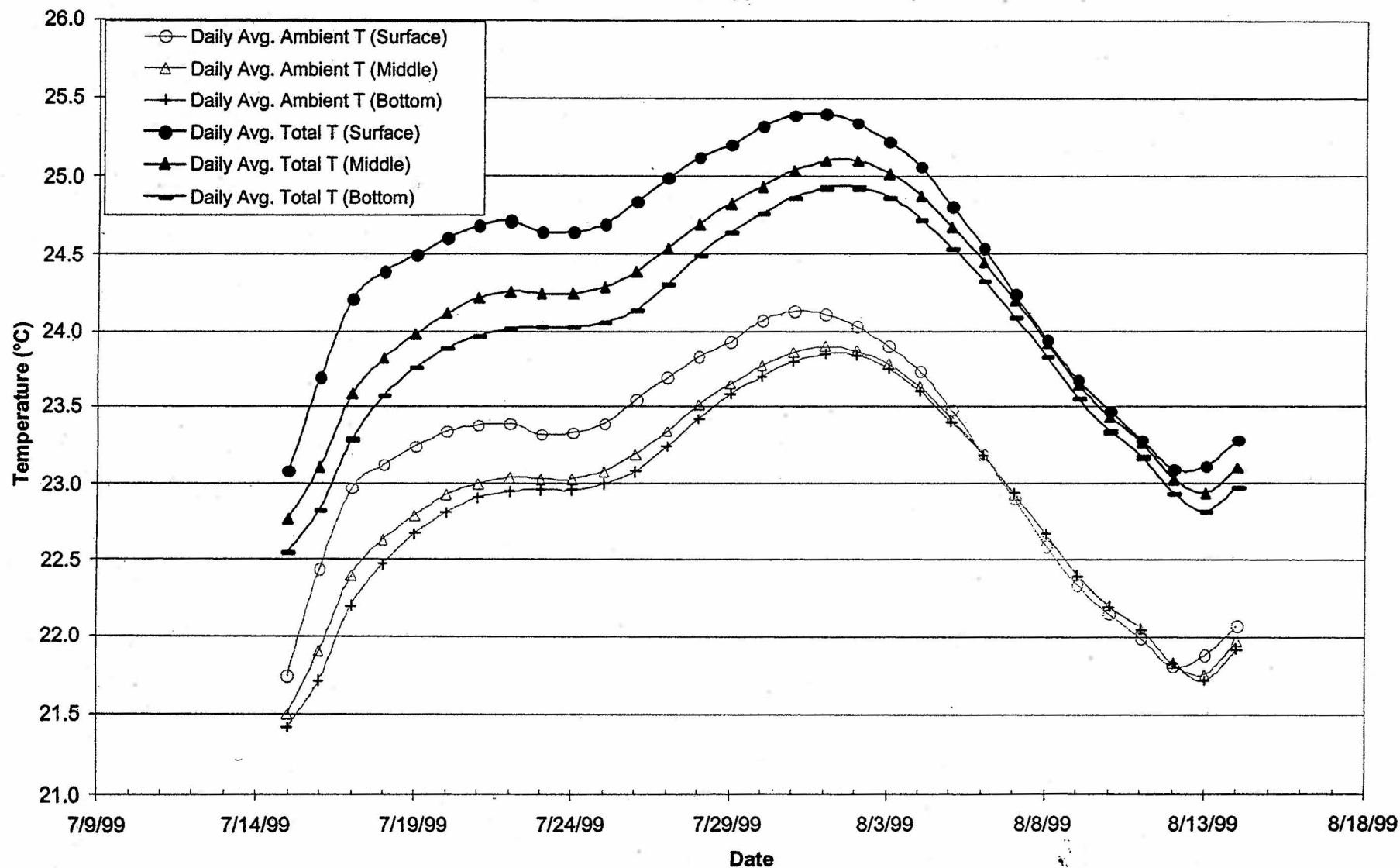
Figure 18: "Translation" of Delta T Results to Avg. range Ambient and Total Temperature (Summer 1999, Hypo B Scenario)
