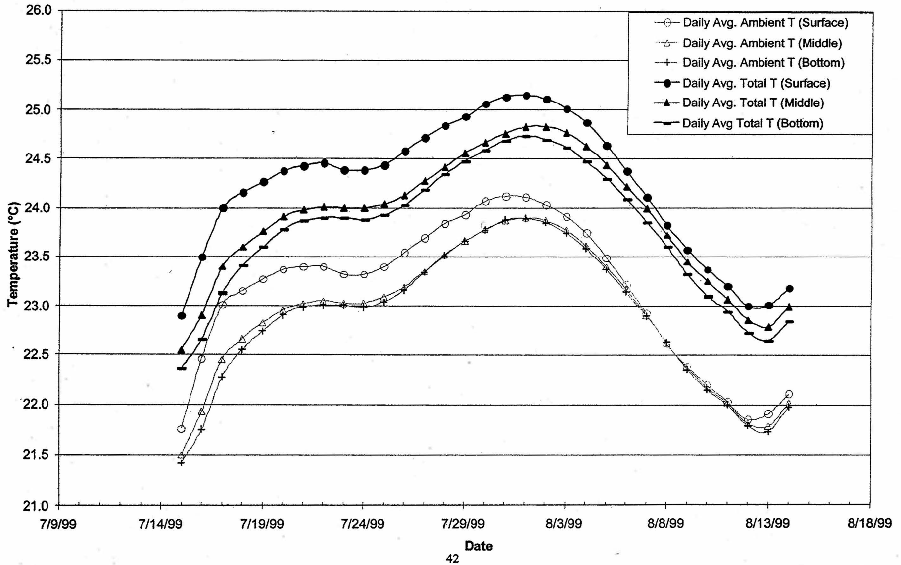
Figure 19: "Translation" of Delta T Results to Average Ambient and Total Temperature (Summer 1999, Hypo A Scenario)
