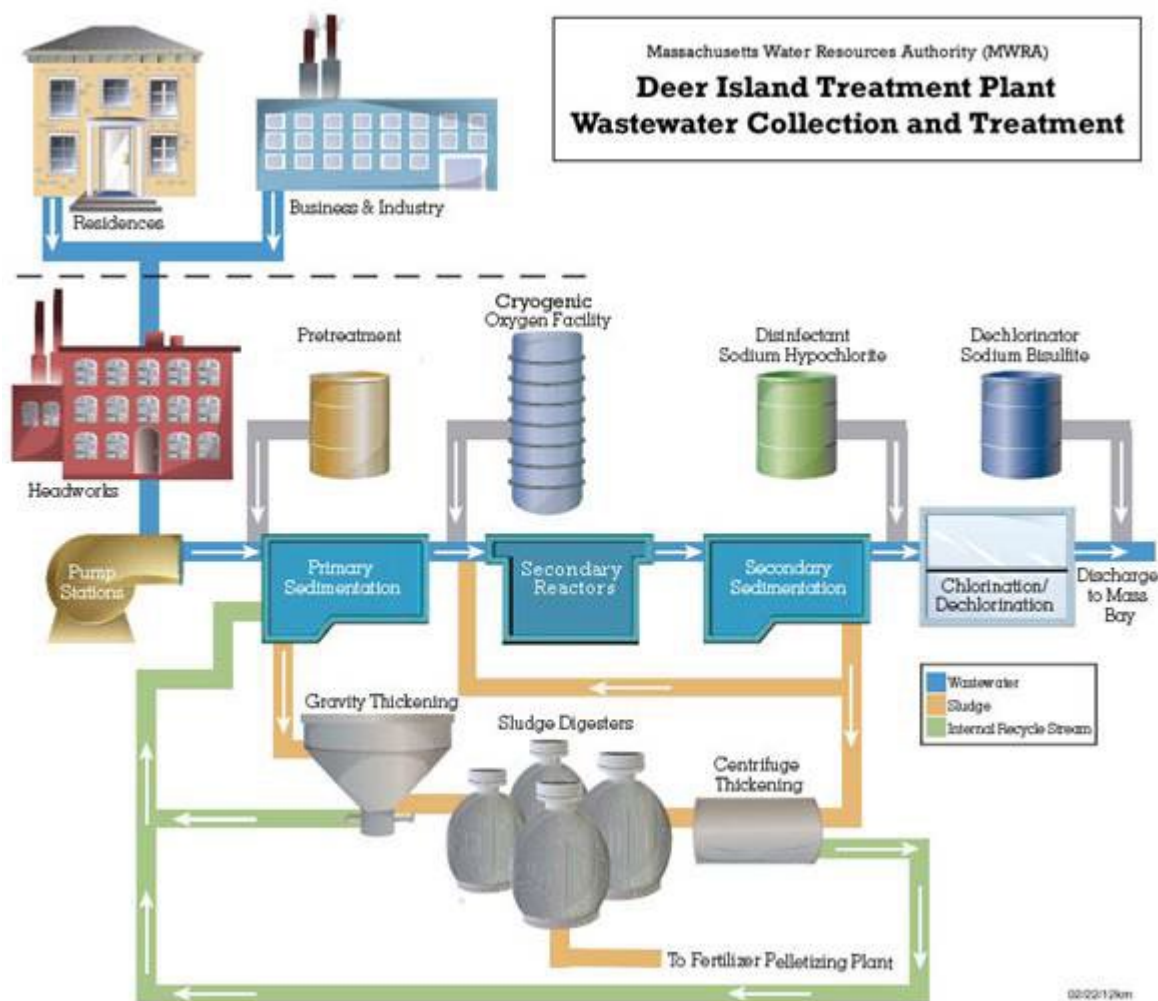
Figure 1. Diagram of the MWRA Deer Island wastewater treatment plant collection and discharge system (courtesy of B. Reilley, 2021, MWRA).
