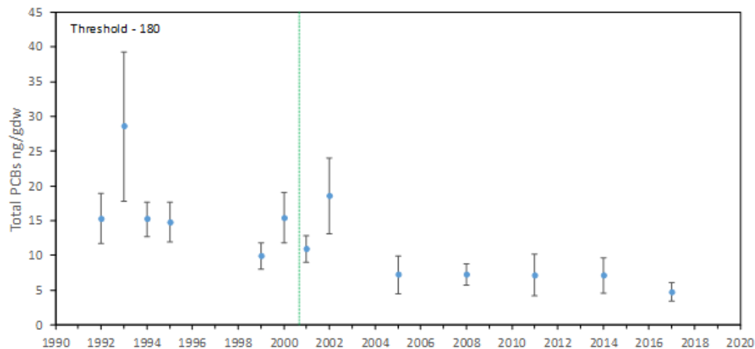
Figure 2. Average Total PCB concentrations (+/- 1 standard error) in nearfield sediments 1992-2017. Dotted green line marks outfall start up.
