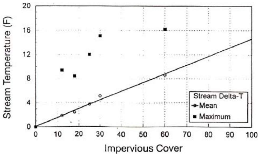
Figure 26: Stream Temperature Increase in Response to IC in Maryland Piedmont Streams (Galli, 1990)
