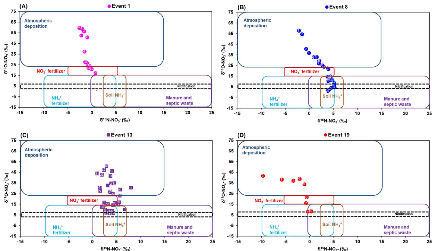
Fig 5. \delta^{15}\text{N}-\text{NO}_3^- and \delta^{18}\text{O}-\text{NO}_3^- in four individual storm events (A) event 1 (number of samples, n = 14 ), (B) event 8 ( n = 27 ), (C) event 13 ( n = 39 ), and (D) event 19 ( n = 10 ) from May to September, 2016.
