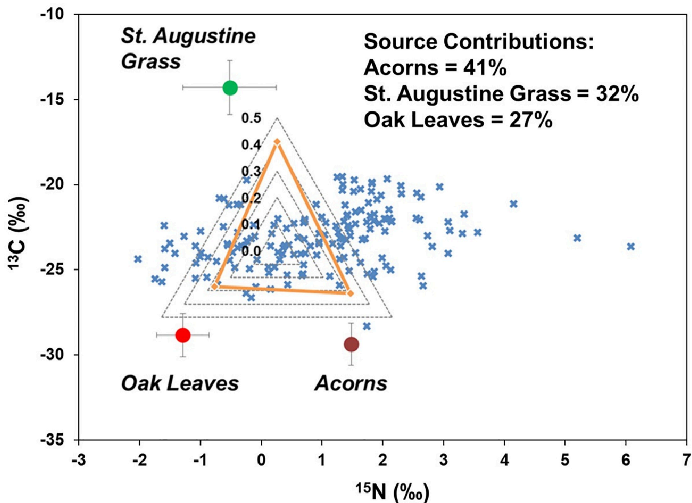
Fig 7. Values of \delta^{15}\text{N} and \delta^{13}\text{C} for particulate organic N (PON) in stormwater runoff samples (blue crosses) and end-members (acorns, oak leaves, and St. Augustine grass). Source proportions of three end-members were derived from the IsoError mixing model and are estimates of the proportion of each source to PON in the stormwater runoff samples.
