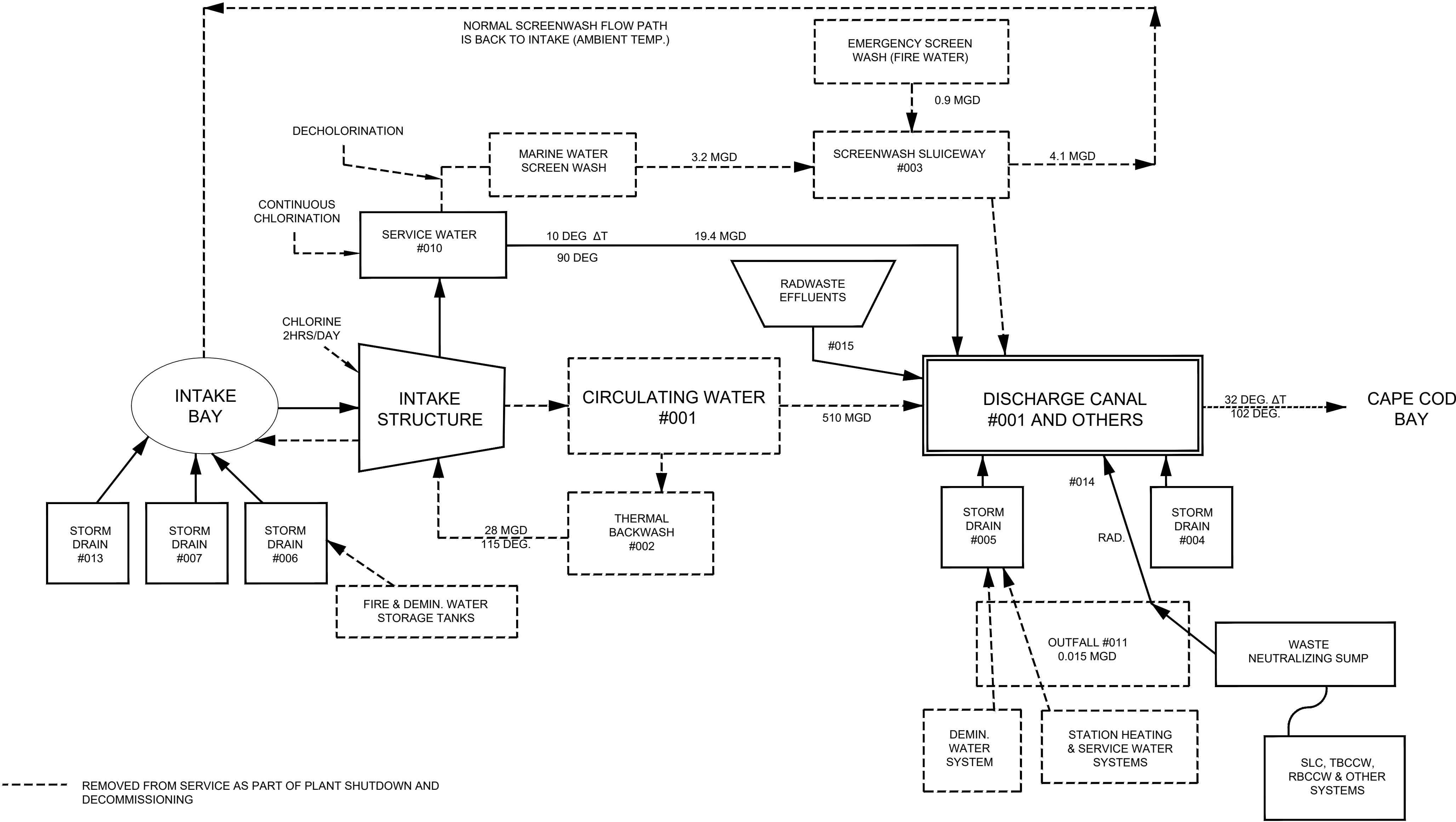
WATER FLOW DIAGRAM PILGRIM NUCLEAR POWER STATION PLYMOUTH, MA
